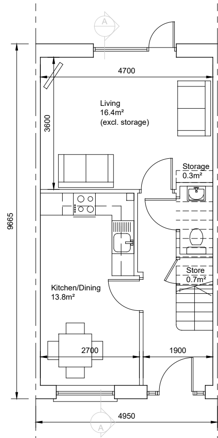
Ground Floor 42.0sqm Total Floor Area 84m 2
