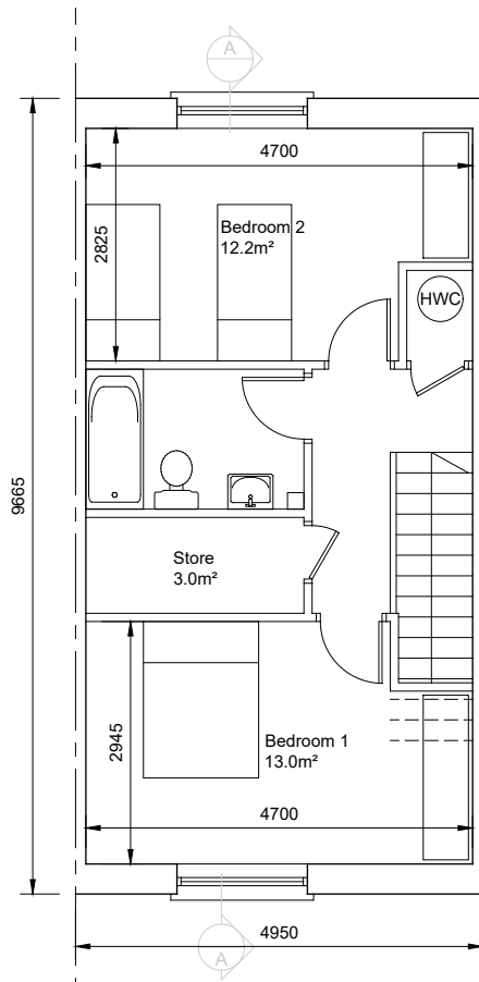
First Floor 42.0sqm
